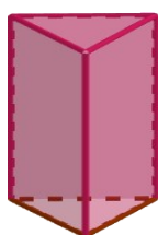
Prisma triangular (irregular)
