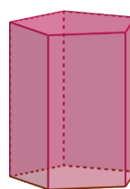
Prisma pentagonal (irregular)
