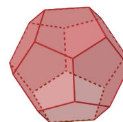
Dodecaedro (regular)
