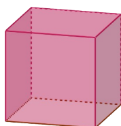
Cubo (regular)
