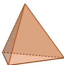
Tetraedro (regular)
