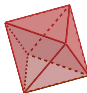
Octaedro (regular)
