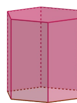
Prisma hexagonal (irregular)
